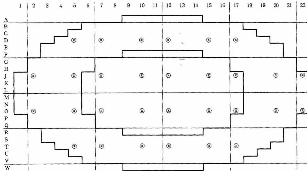
FIGURE 3. LOCATION OF FRESH FUEL FOR 30 AGE PATTERNS
