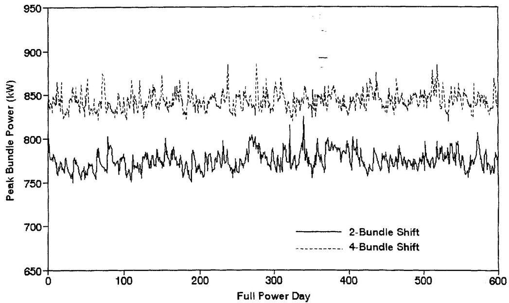
FIGURE 5. COMPARISON OF PEAK BUNDLE POWER(KW)
