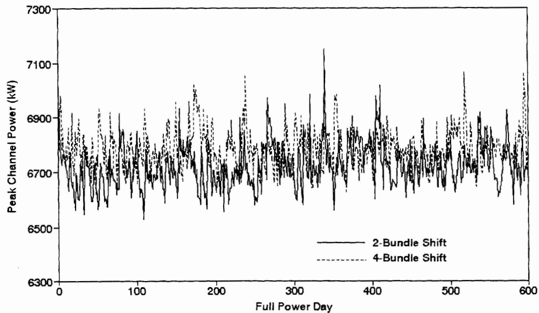
FIGURE 4. COMPARISON OF PEAK CHANNEL POWER(KW)
