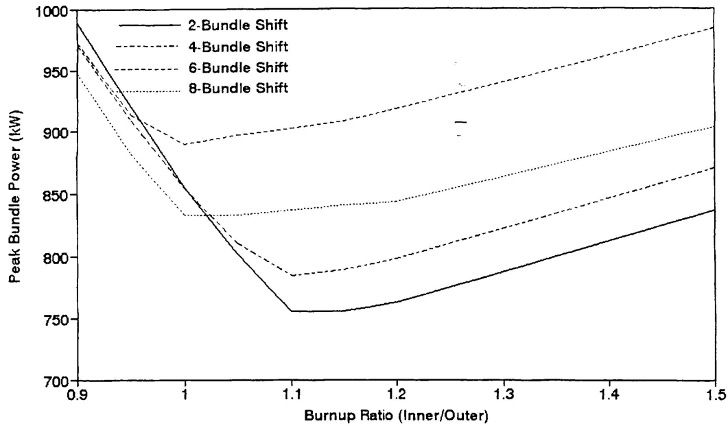
FIGURE 1. MAXIMUM BUNDLE POWER(KW) FOR EACH REFUELING SCHEME
