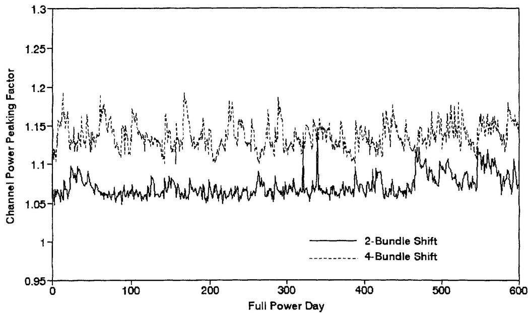
FIGURE 6. COMPARISON OF CHANNEL POWER PEAKING FACTOR
