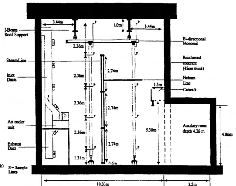
Figure 2: A schematic of the facility (a view of the south wall, from the north wall).
