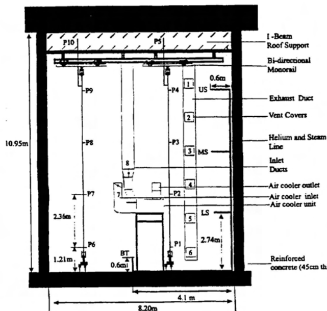
Figure 1: A schematic of the facility (a view of the east wall, from the west wall).
